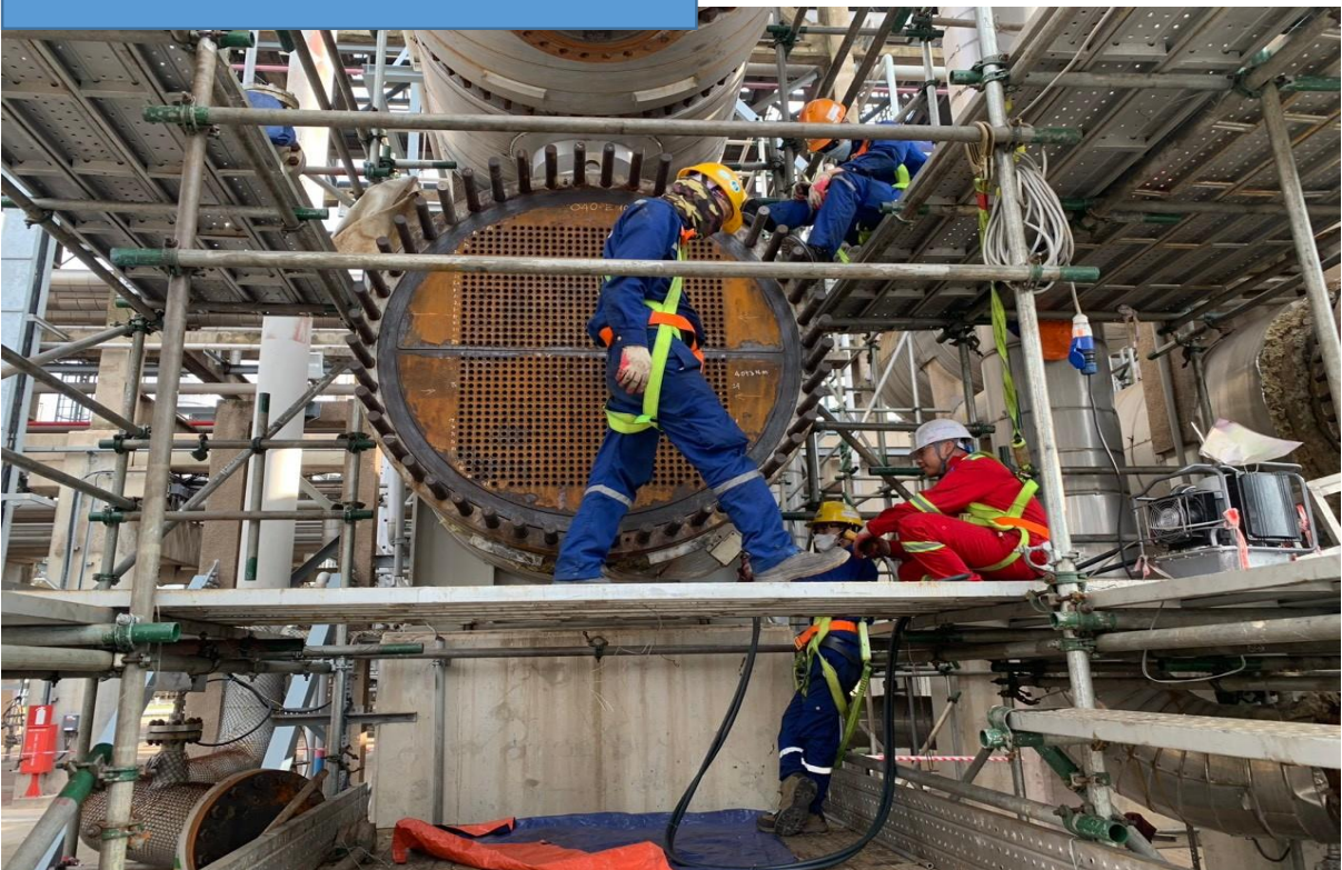
REMOVING CHANEL HEAD
