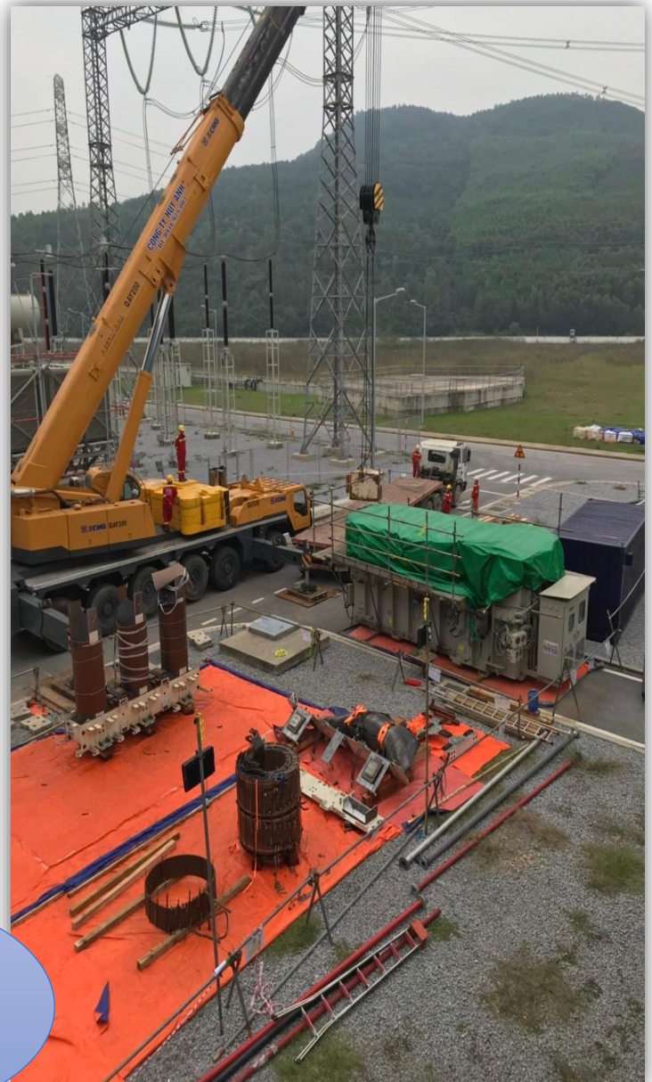
Unloading and dismantling transformer
