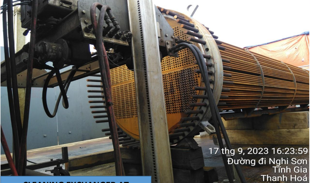
CLEANING EXCHANGER AT WASHING BAY
